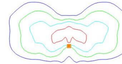
KIM ERA LANTERN 10 FOOT TALL POLE TYPE III OPTIC FOR ROADS PRODUCT USED AT STRAWBRIDGE
